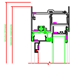
100 HEAD SERIES 3000
