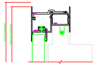
101 HEAD SERIES 3000
