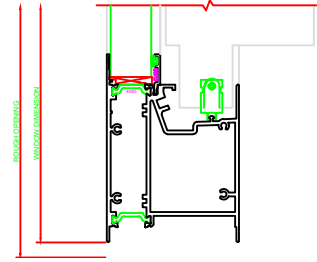
201 SILL SERIES 3000
